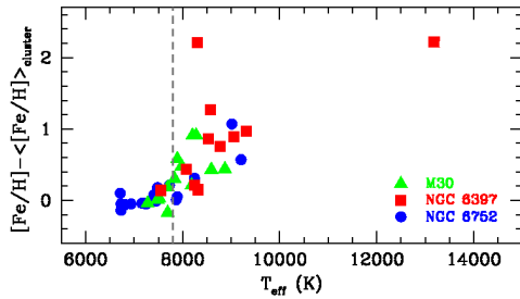
Fig. 2. [Fe/H] ratios (scaled on the mean cluster iron content) as a function of stellar temperatures for the BSS samples of M30, NGC 6397 and NGC 6752.
