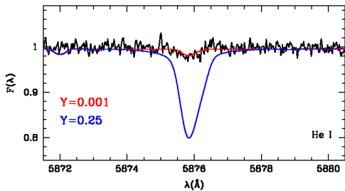
Fig. 1. He I line at \sim 5876 Å for a BSS of NGC 6397.
